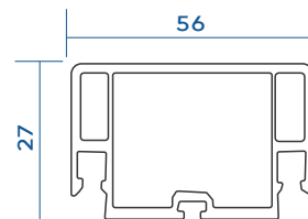
Mesh Mullion VGA-620-MT1
