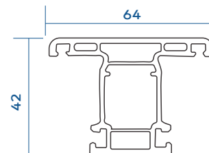
Sash Mullion VGA-620-T01
