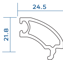
Sliding Single Glazing Arch Bead 5/6 MM With Gasket VGS-181-B01
