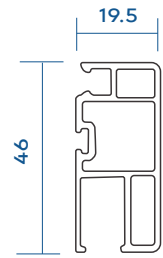
Sliding Window Mesh Sash VGS-500-M01
