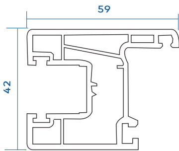
Sliding Window Sash With Gasket VGS-621-S01
