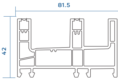
Sliding Outer Frame 2.5 Track With Mesh VGS-500-F02
