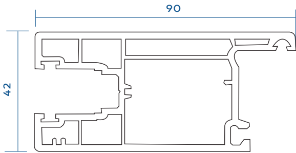
Sliding Door Sash With Gasket VGS-621-S04
