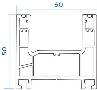
2 Track Sliding Outer Frame VGS-620-F01
