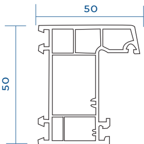
Casement Window Outer Frame With Gasket VGC-501-F01
