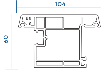
Casement Outward Opening Door Sash With Gasket VGC-601-S02
