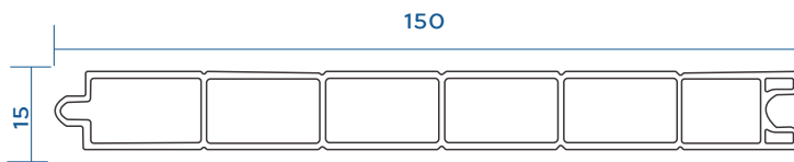
Panel 15 Mm Profile 150 Mm VGA-160-A02
