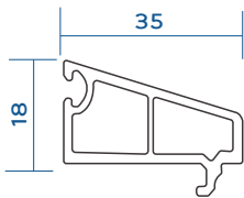
Casement Single Glazing Bead 5/6 Mm With Gasket VGC-181-B02
