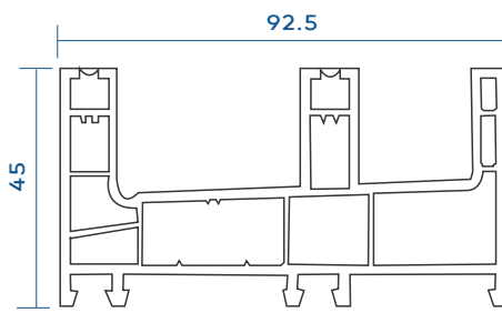
Sliding Outer Frame 2.5 Track With Mesh VGS-620-F02
