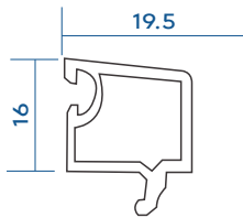
Sliding Single Glazing Bead 5/6 Mm With Gasket VGS-181-B02
