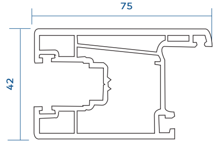
Sliding Super Big Sash With Gasket VGS-621-S03
