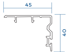
Sliding Inter Lock VGS-621-L01
