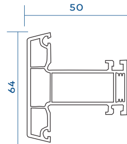
Casement T Mullion With Gasket VGC-601-T02
