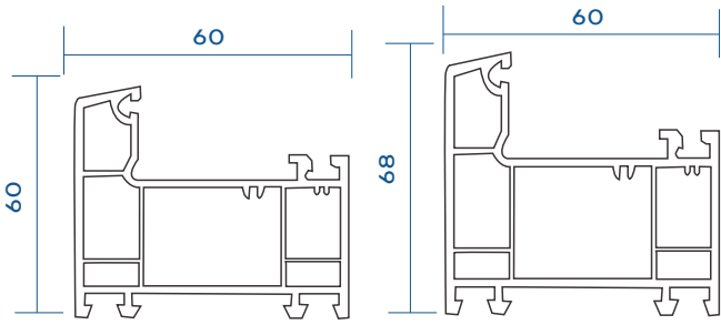
Casement Window Outer Frame With Gasket VGC-601-F01
