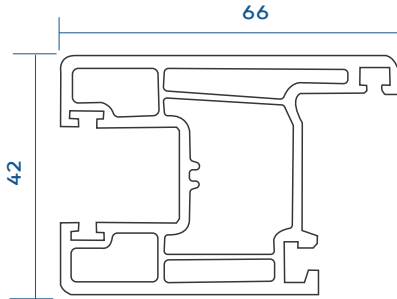
Sliding Window Super Sash With Gasket VGS-621-S02
