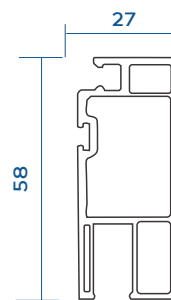
Sliding Window/Door Mesh Sash VGS-621-M01
