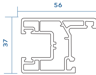
Sliding Window Sash With Gasket VGS-501-S01
