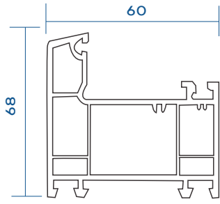
Casement Door Outer Frame With Gasket VGC-601-F02
