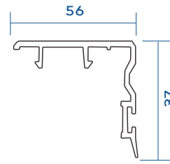
Sliding Inter Lock VGS-500-L01
