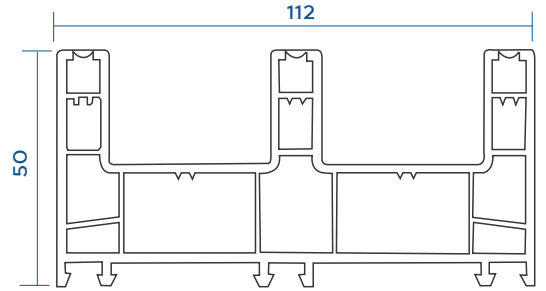
Sliding Outer Frame 3 Track VGS-620-F03
