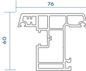
Casement Outward Opening Window Sash With Gasket VGC-601-S01
